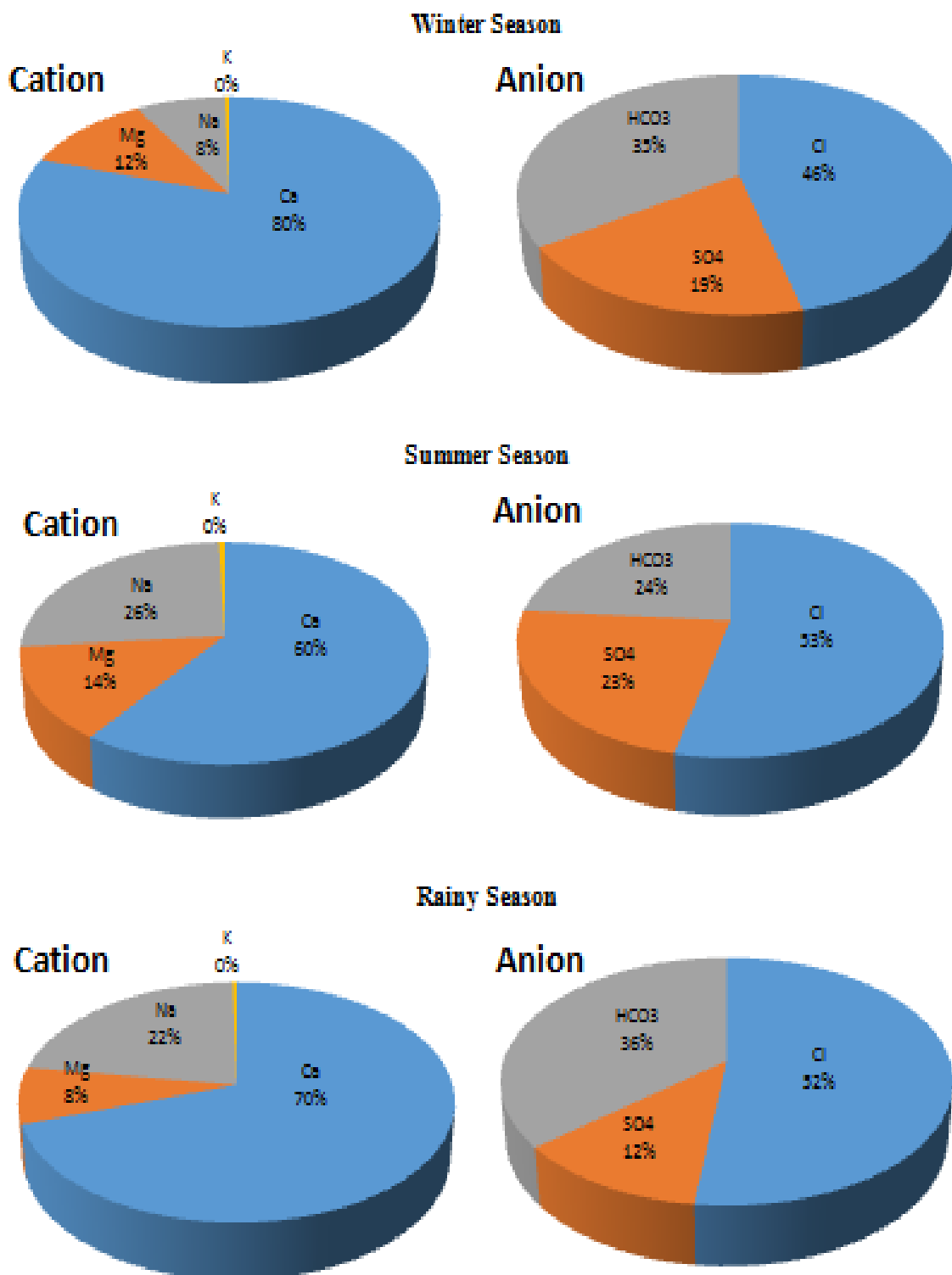
Figure 2. Pie diagram of mean values of major ions during the study period
